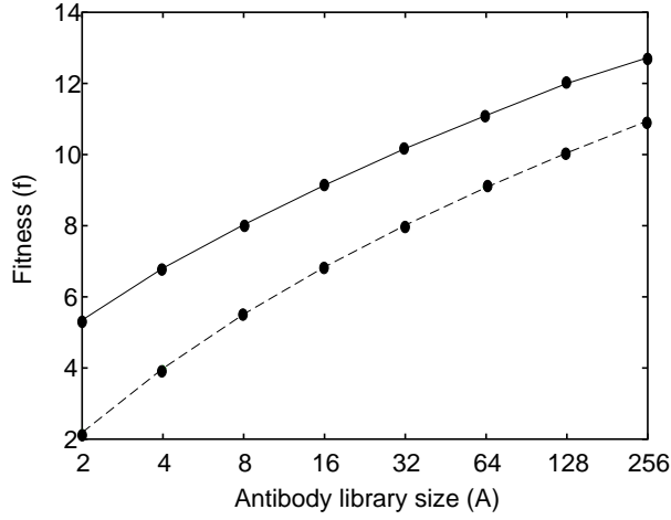
Figure 1: Scaling Of Fitness On A Random Pathogen Set With The Antibody Set Size A . The solid line shows the fitness of the best library evolved in 1000 steps of the genetic algorithm, and the dashed line the expected fitness of a random library. For the solid line, the points on the curve are averages over 100 (for library size A = 2, 4, 8, 16, 32, 64 ) or 10 (for library size A = 128 and 256 ) independent runs, in which we took the best fitness in the population at the end of the run. The line is obtained by interpolating between these points.
