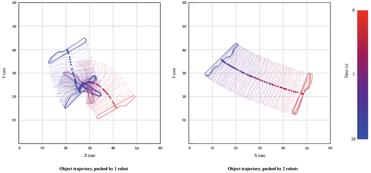
Figure 10: Comparison of object trajectories when pushing a knife with one robot versus two robots. Trajectories are color-coded by time, as indicated by the color bar to the right of the figure. Dots represent the moving object’s center point at various moments.
