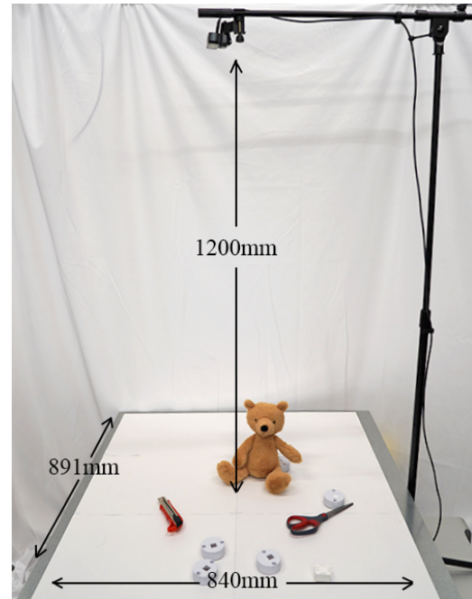
Figure 3: Hardware setup of Push-That-There
