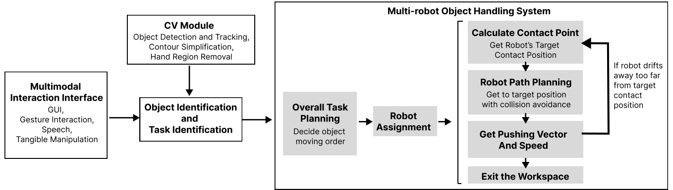
Figure 4: System software pipeline
