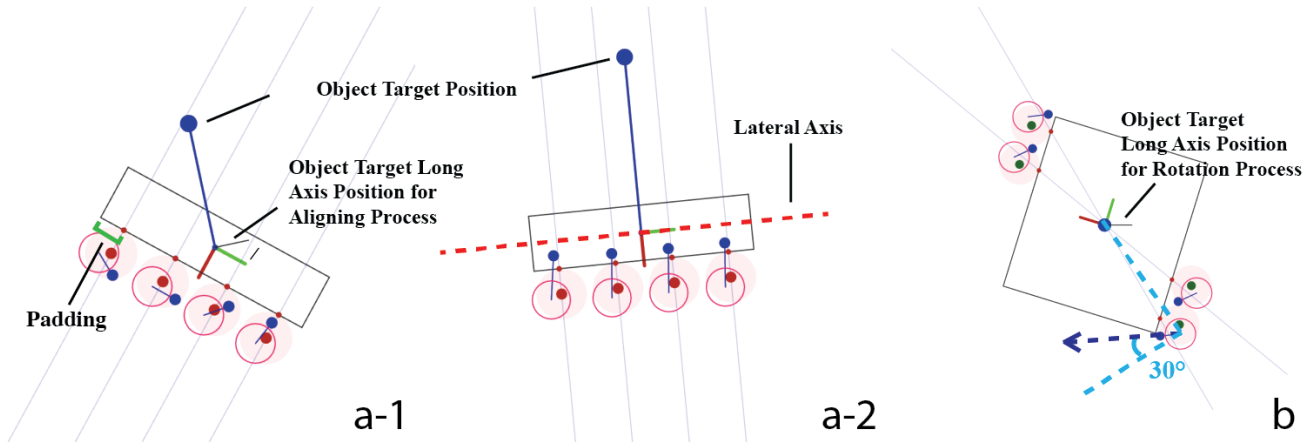
Figure 5: Contact points and robot's pushing vector calculation illustration. (a) Aligning (be prepared to push) process and pushing process. (a-1) Aligning the long object to the optimized pushing orientation before pushing. (a-2) Pushing the object. We use our novel lateral axis (represented by the dashed red line) alignment control to adjust the robot's speed. (b) Rotating the object. We calculate the pushing vector for robots using the vector that is 30° inward of the object from the vector obtained by subtracting the object's center from the robot's position.
