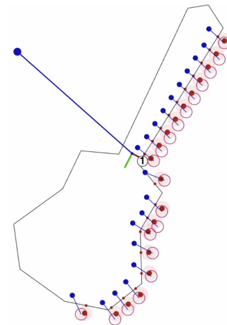
Figure 15: Simulation of our robot assignment algorithm with larger objects and more robots. In this figure, we are assigning 20 robots to push a guitar.
